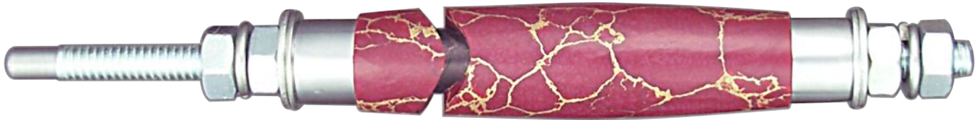
Single Wave Milled for Phoenix Rising Twist Pen in TruStone Maroon and Gold Matrix After Milling Channel for Crushed Opal Inlay with CNC Rotary Table (PSI PKRISEAB & PSI WXTS2134)
