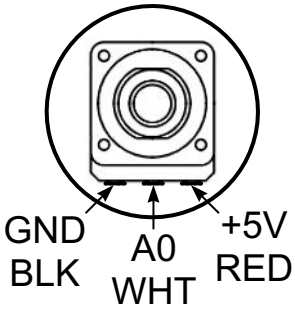
250Ω Potentiometer Wiring Top View
