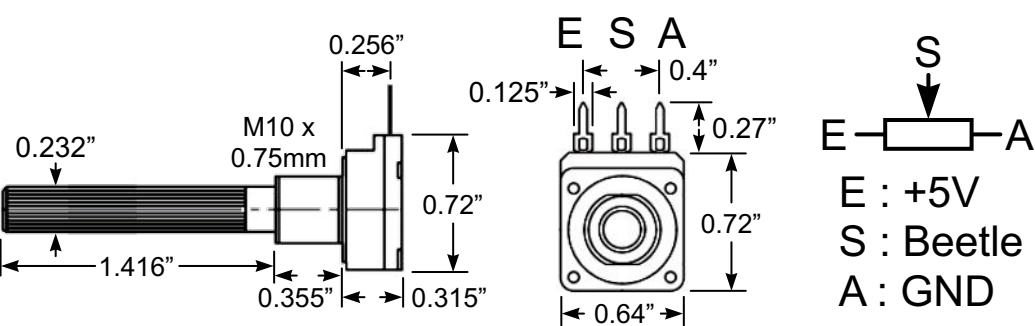
250Ω Potentiometer with 45mm Adjustment Post Length (ESA Connections As Seen From Post Side)
